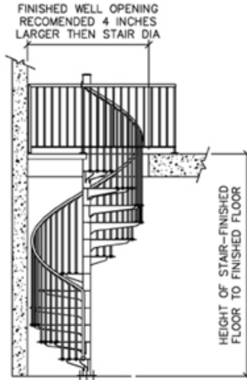
FINISHED WELL OPENING RECOMENDED 4 INCHES LARGER THEN STAIR DIA HEIGHT OF STAIR-FINISHED FLOOR TO FINISHED FLOOR BASE PLATE ANCHORED TO FINISHED FLOOR OR BELOW FLOOR LEVEL
