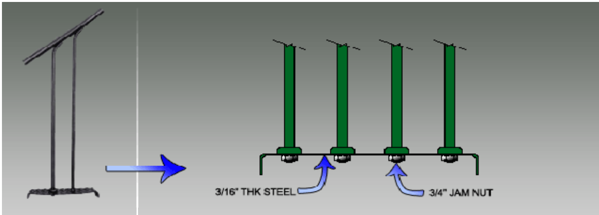
Baluster attachment on a No. 111, No. 131, No. 135, No. 175 Tread Designs
