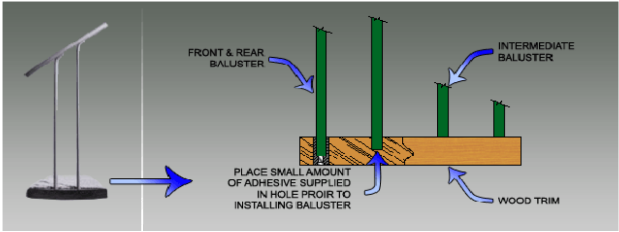
Baluster attachment on a No. 165 Tread Design
