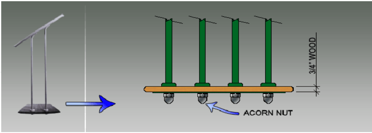
Baluster attachment on a No. 141 Tread Design
