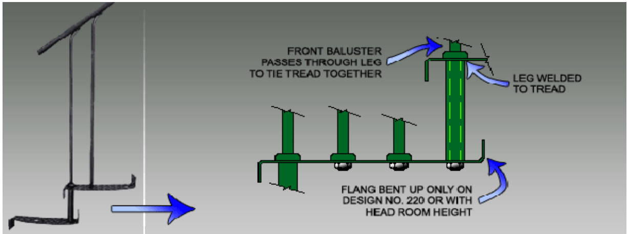
Baluster attachment on a No. 201, No. 220, No. 251, and No. 320 Tread Designs
