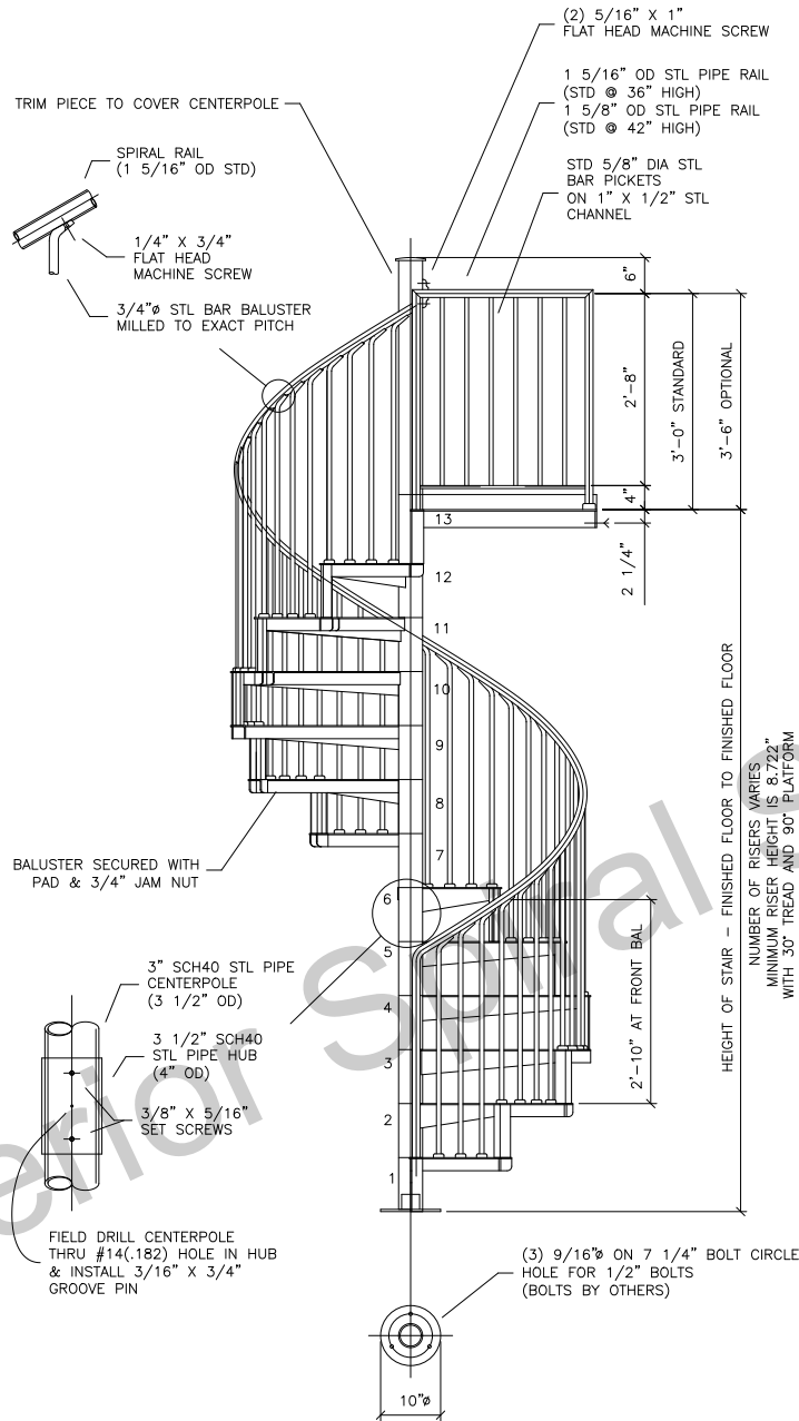
TYPICAL ELEVATION
